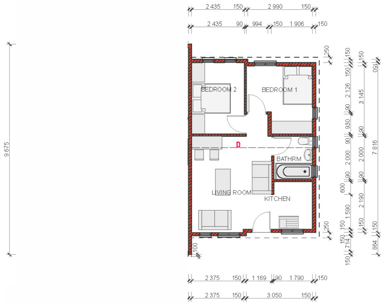
GROUND FLOOR PLAN - 46m 2
