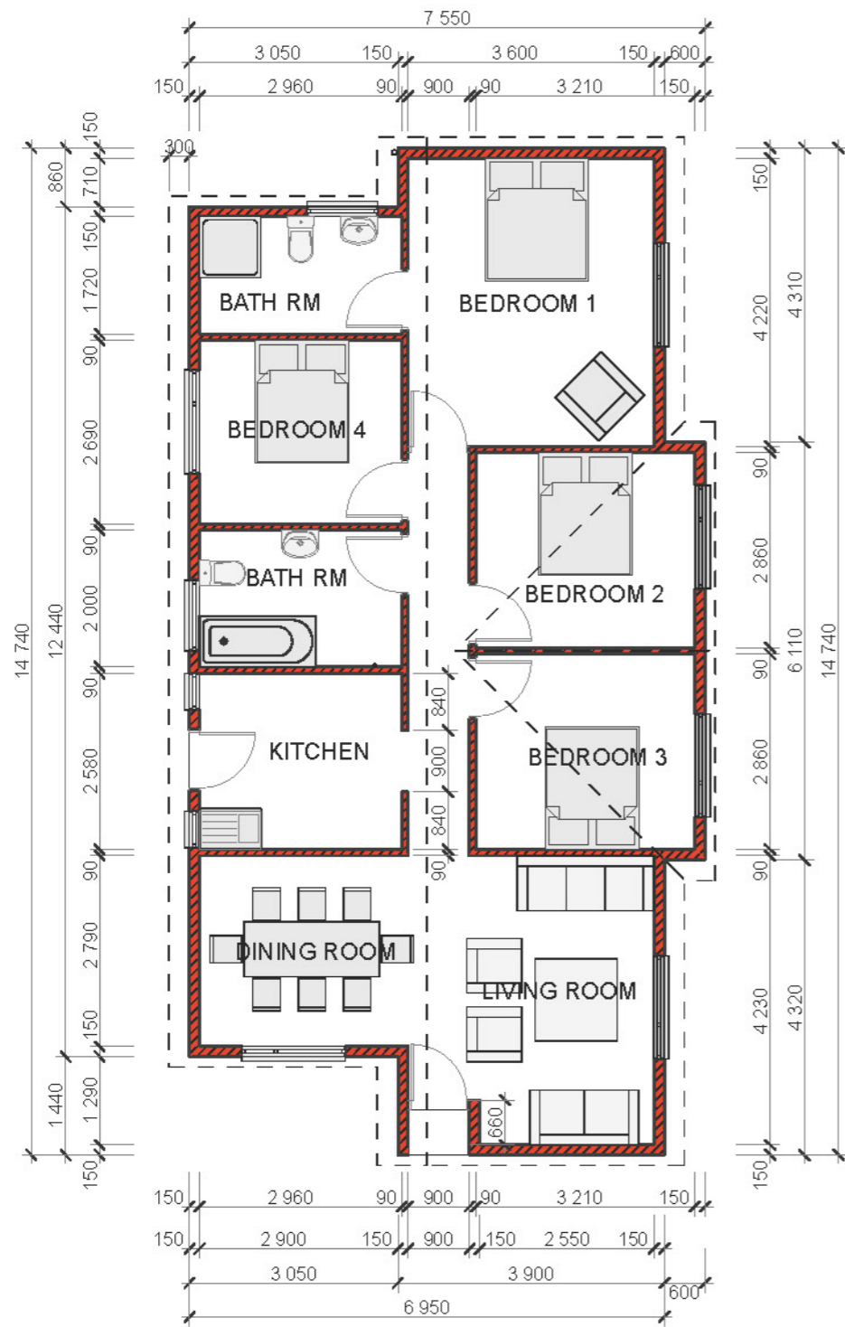
GROUND FLOOR - 99m 2
